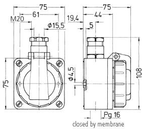
Drawing 1 MB 347 Dim. in mm
